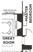
Optional Fireplace At Master Bedroom Entry
