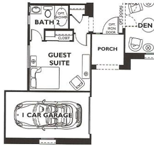
Optional 1 Car Garage At Elevation 'A'
