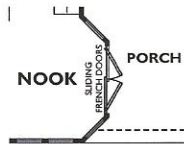
Optional Sliding French Doors At Nook (Elevation 'A' & 'B' only)
